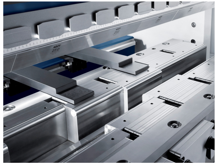
EHT VarioTool – a flexible lower tool for dies of 120 to 300 mm.
