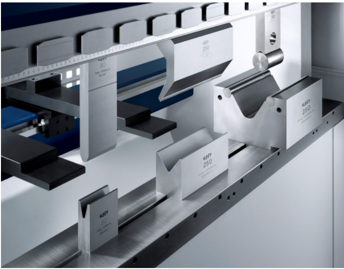
A flexible tool system for individual V dies and the VarioTool.
